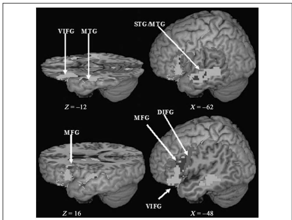
Figure 4. Activation map for the meaning task and the rhyming task in the auditory modality. Green indicates the activation for the meaning task; red indicates the activation for the rhyming task; blue indicates the overlapping activation for both tasks.
