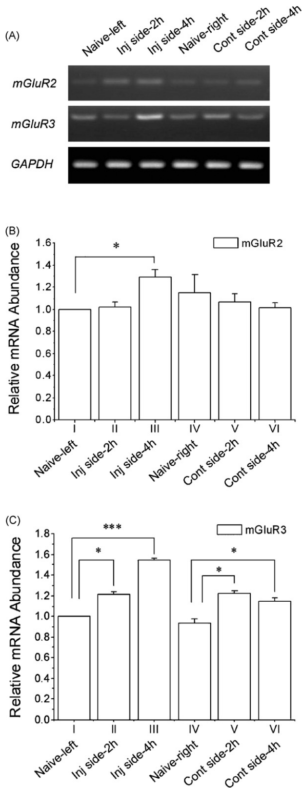
Fig. 1. Relative mRNA expression of rmGluR2 and rmGluR3 in the spinal cord. (A) Electropherogram images shown rmGluR2 and rmGluR3 expression in the spinal cord under naive, 2 and 4 h after CFA treatment (left side hind-paw) states based on semi-quantitative real-time PCR. In the spinal cord, quantitative real-time PCR displays that mRNA expression level of rmGluR2 (B) is up-regulated 4 h after s.c. CFA injection; but that of rmGluR3 (C) is up-regulated 2 and 4 h after CFA treatment at the injected side and control side. The y-axis represents the relative intensity of mRNA expression. The value of each gene mRNA expression in the left side of naive is designated 1, and the levels of mRNA expression in other samples are calibrated to this value. * p < 0.05 ; *** p < 0.0001 .
